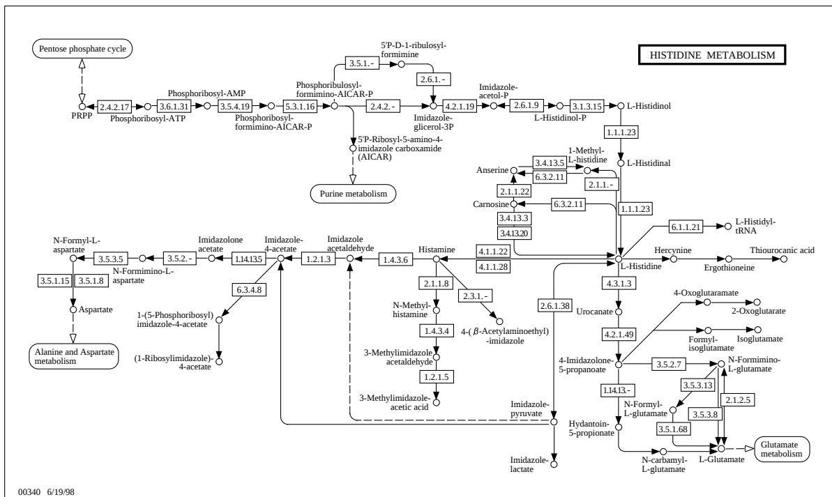
Figure 1: The KEGG standard pathway map for histidine metabolism.
